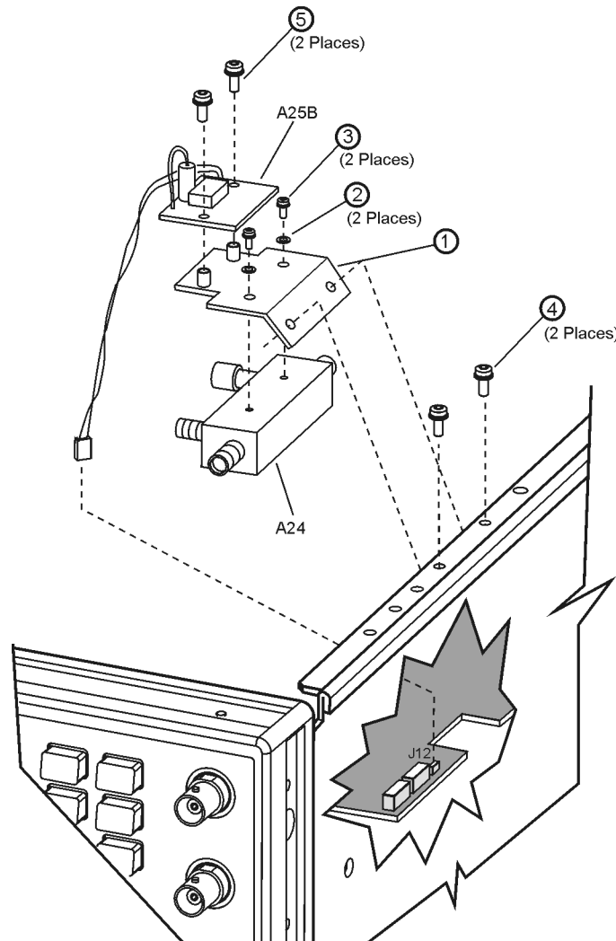
Figure 3-29 Disassembled A24 20 GHz High Band Coupler and A25B Highband Detector Bias Board
