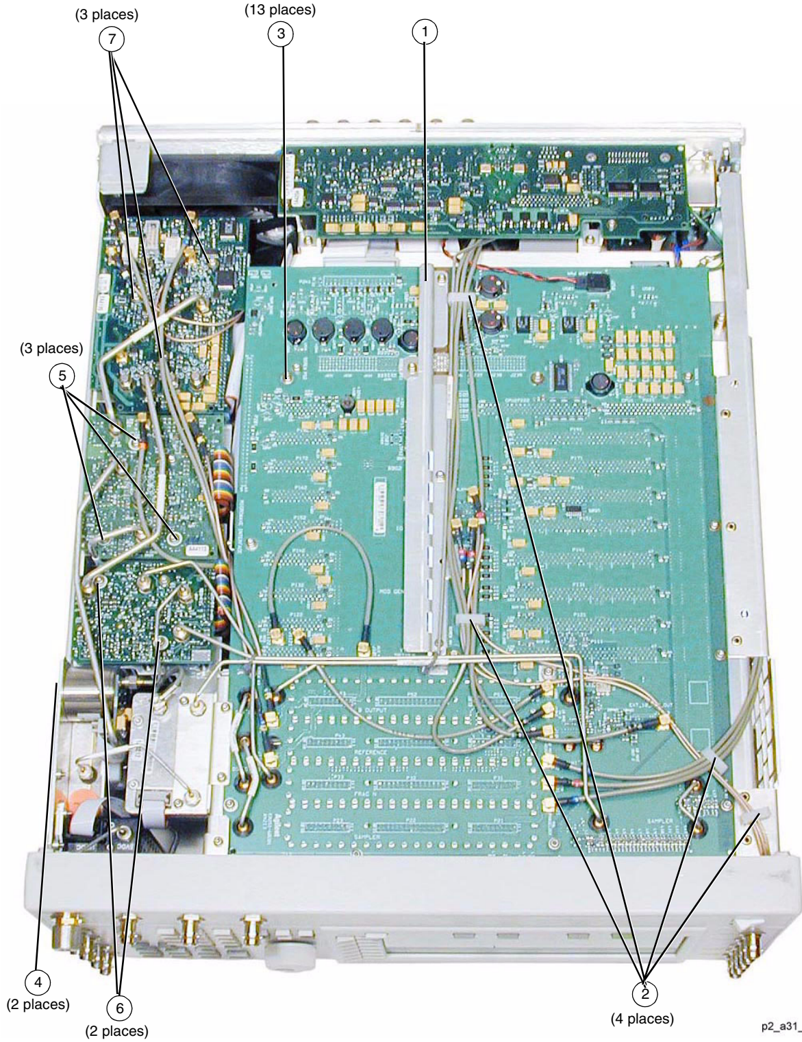
Figure 3-34 Main Chassis and MID Bottom View (E8267C)
