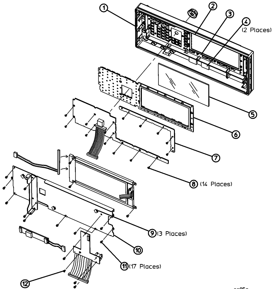
Figure 3-24 Disassembled Front Panel View
