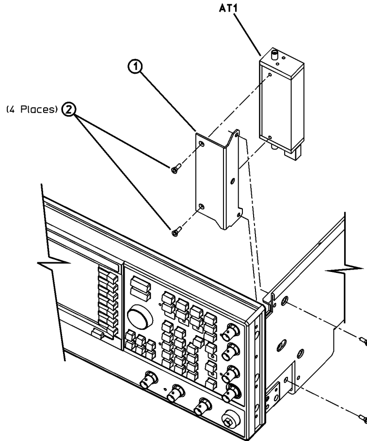
Figure 3-28 Disassembled AT1 115 dB Attenuator View (Option 1E1)
