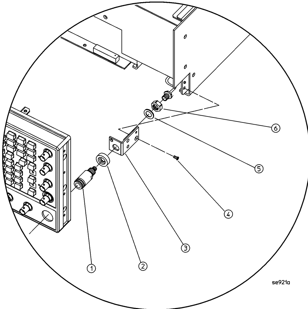
Figure 3-37 Type-N RF Output Connector (Option 1ED Models Only)
