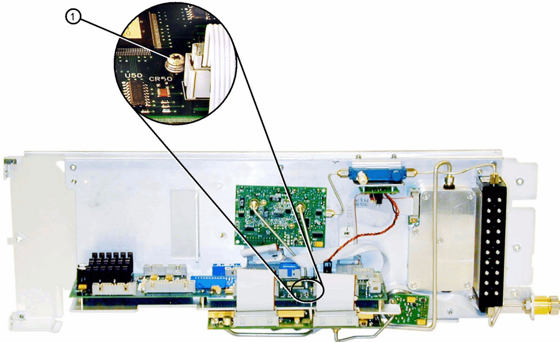
Figure 3-31 E8247C/57C Microcircuit Interface Deck Top View
