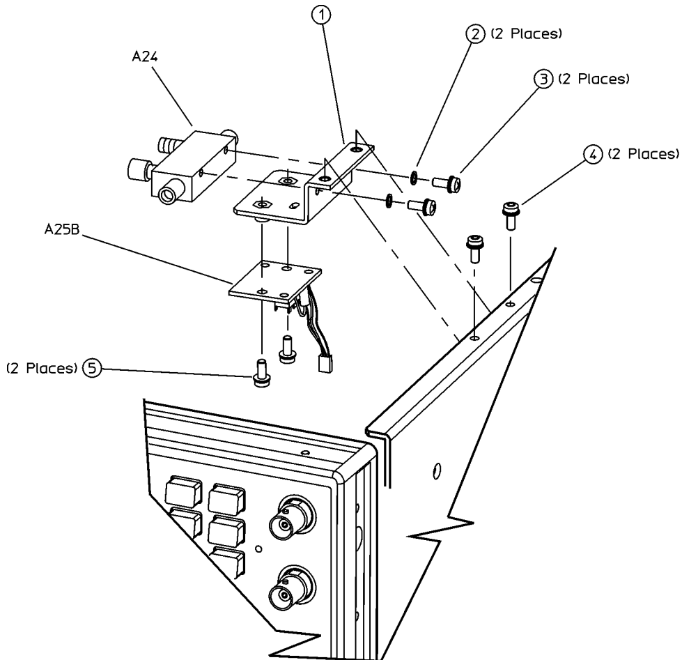
Figure 3-30 Disassembled A24 40GHz High Band Coupler and A25B High Band Detector Bias Board
