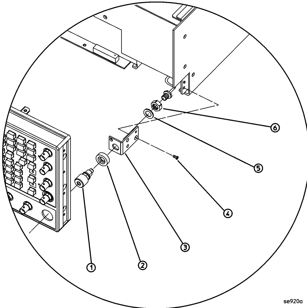
Figure 3-36 APC 3.5 RF Output Connector (Option 520 Only)
