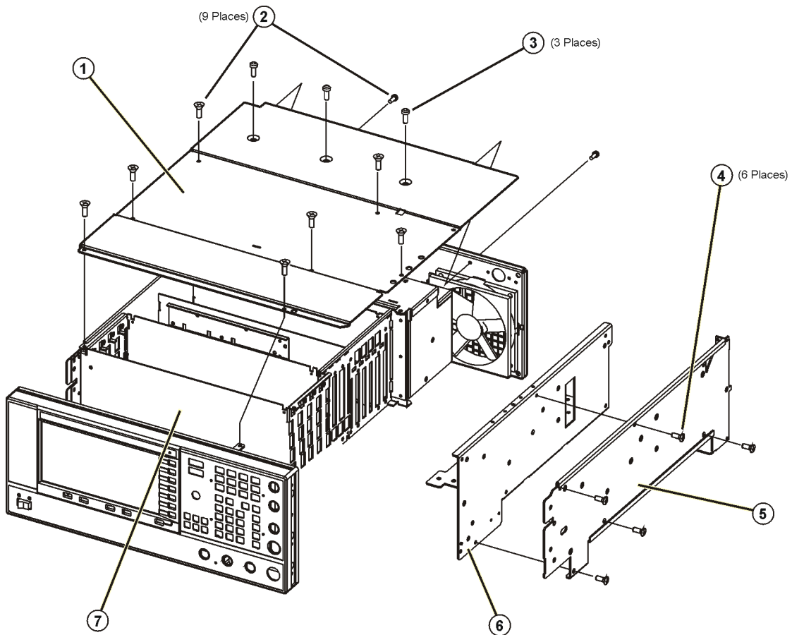
Figure 3-38 Main Chassis with Inside Cover and Right-Side Support Wall
