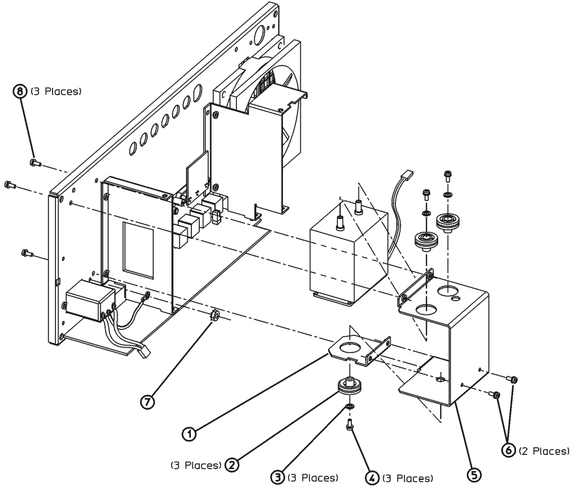
Figure 3-27 Disassembled A32 10 MHz Crystal Oscillator (Option UNR)
