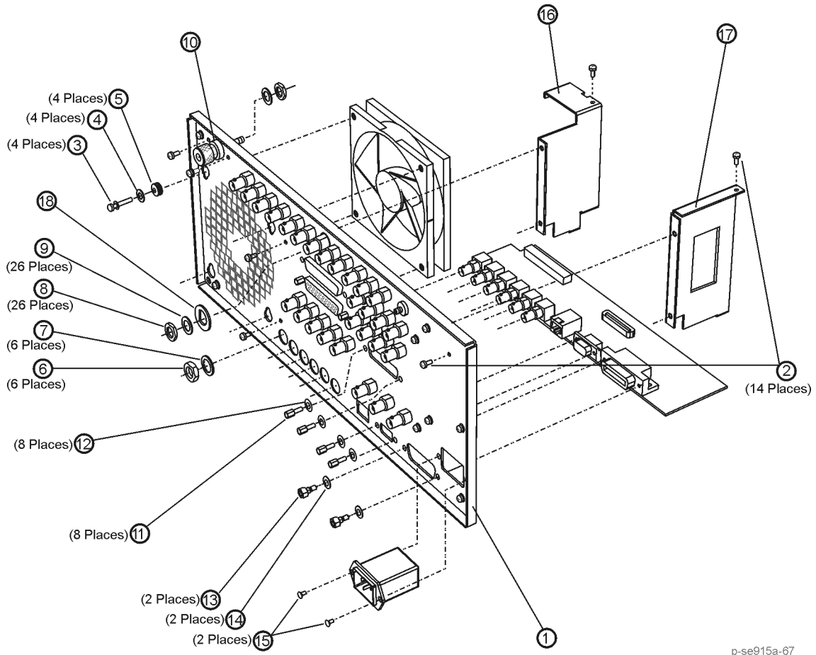
Figure 3-26 E8267C Disassembled Rear Panel View
