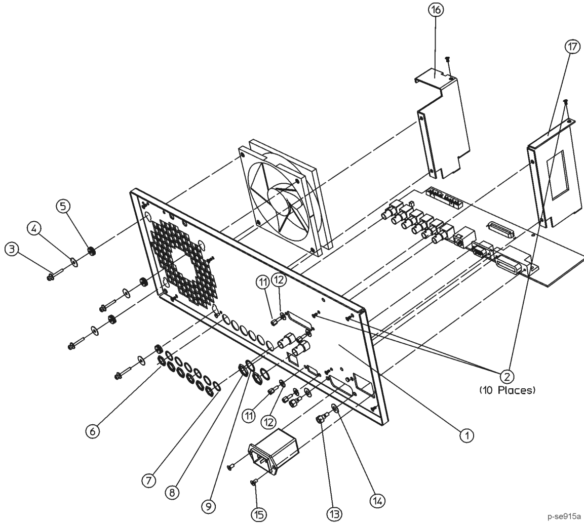
Figure 3-25 E8247C/57C Disassembled Rear Panel View
