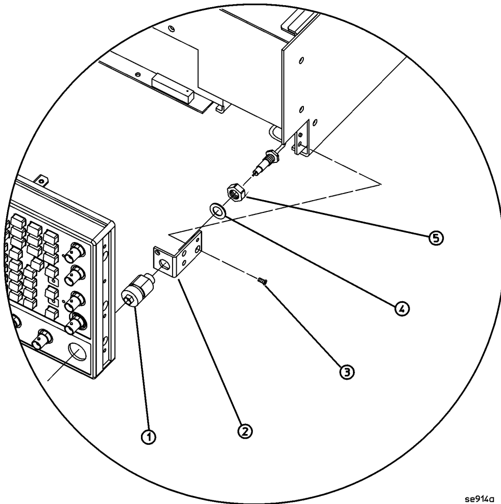
Figure 3-35 2.4 mm RF Output Connector (Option 540 Only)
