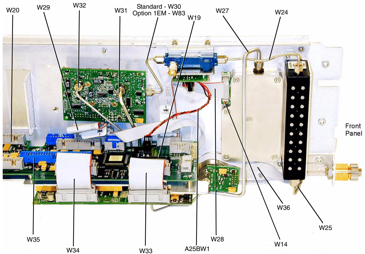
Figure 3-18 E8247C and E8257C (Option 540) MID
