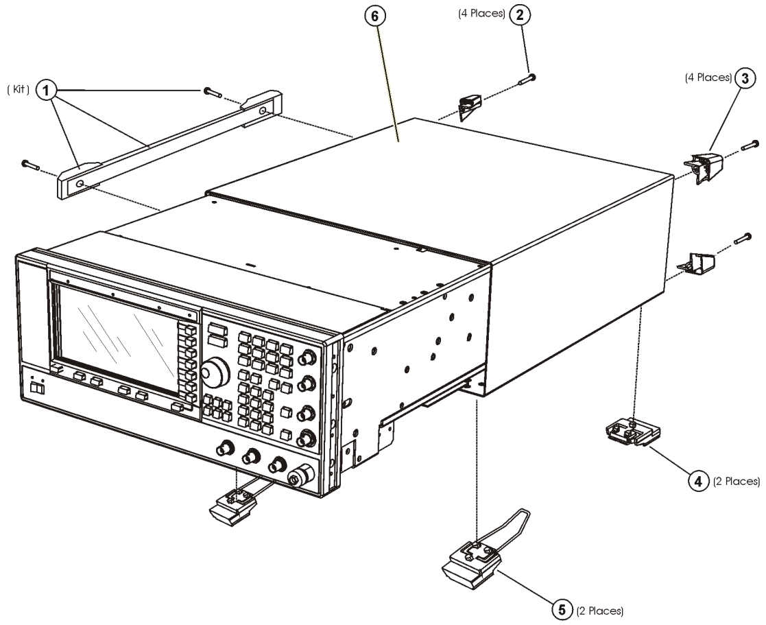
Figure 3-39 Outer and Inner Instrument Covers and Associated Parts
