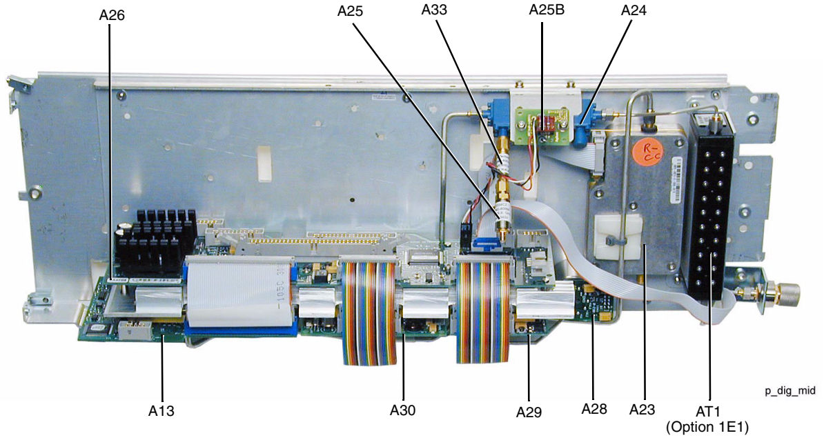
Figure 3-8 Assemblies from a Microcircuit Deck View (E8267C Option 520)
