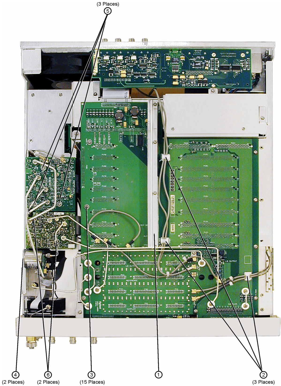
Figure 3-33 Main Chassis and MID Bottom View (E8247C/57C)
